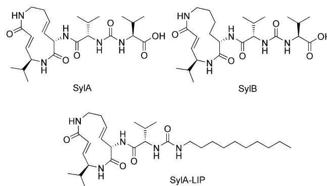
Figure 1. Chemical structures of the natural product proteasome inhibitors syringolin A (SylA), syringolin B (SylB), and synthetic derivative SylA-LIP.
