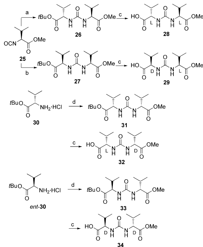
Scheme 8. Synthesis of all four stereoisomers of the urea building blocks. Reagents and conditions: (a) 30 (1 equiv.), DIEA (2 equiv.), DCM, room temp., overnight, 90%; (b) ent - 30 (1 equiv.), DIEA (2.5 equiv.), DCM, room temp., 1 h, 91%; (c) wet HCO 2 H, 28 : 91%, 29 : 91%, 32 : >98%, 34 : 92%; (d) triphosgene (1.1 equiv.), DIEA (2.2 equiv.), DCM, 5 min at room temp. then ( D )-valine methyl ester hydrochloride (1 equiv.), DIEA (2.2 equiv.), DCM, 10 min at room temp., 31 : 30%, 33 : 76%.
