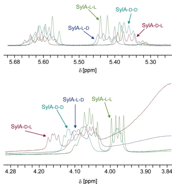
Figure 2. Overlay of the characteristic part of the 1 H NMR spectra of 37a (SylA-L-L), 37b (SylA-L-D), 37c (SylA-D-L), and 37d (SylA-D-D).
