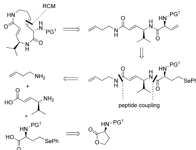
Scheme 4. Retrosynthesis for the generation of the core macrocycle by using ring-closing metathesis (RCM) as a key step.
