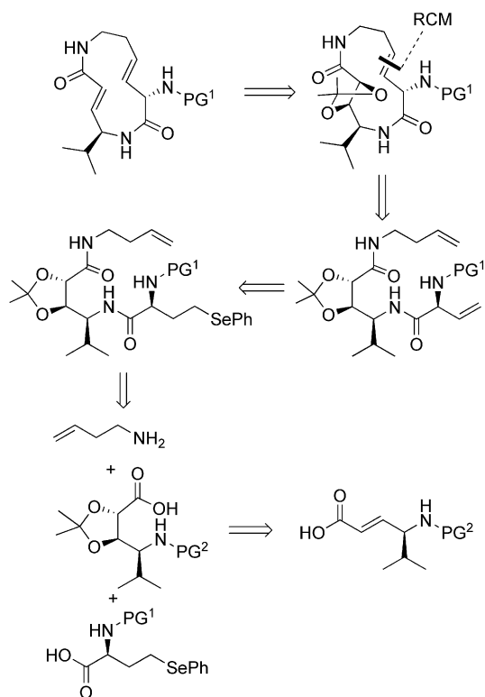
Scheme 6. Retrosynthesis for the generation of the core macrocycle by using ring-closing metathesis (RCM) on a conformationally pre-oriented precursor.
