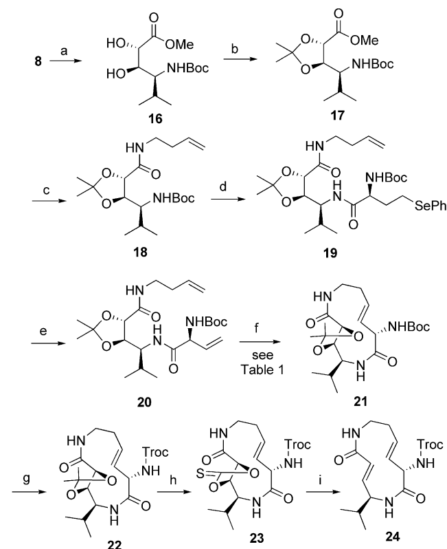
Scheme 7. Synthesis of the SylA macrocycle core structure by using a RCM approach with structural preorganization. Reagents and conditions: (a) OsO 4 (0.05 equiv.), NMO (1.5 equiv.), Ac 2 O/H 2 O (2:1), 48 h at room temp., 85%; (b) 2,2-DMP (30 equiv.), PPTS (0.05 equiv.), DCM, reflux, >98%; (c) 1. 1 M aq. LiOH (3 equiv.), MeOH/H 2 O (1:1), 0 °C to room temp. over 30 min; 2. 3-butenylamine hydrochloride (1.2 equiv.), PyBop (1.5 equiv.), HOAt (1.5 equiv.), DIEA (2 equiv.), DCM, 0 °C to room temp. overnight, 80% (two steps); (d) 1. 2,6-lutidine (2 equiv.), TMSOTf (1.5 equiv.), DCM, room temp., 15 min; 2. 12 (1.3 equiv.), PyBop (1.5 equiv.), HOAt (1.5 equiv.), DIEA (2 equiv.), DCM, from 0 °C to room temp. overnight, 87% (two steps); (e) 30% aq. H 2 O 2 /DIEA (1:1), DCM, 3 h at 50 °C, 93%; (f) Grubbs II catalyst (0.15 equiv.), toluene, 18 h, 90 °C, 49%; (g) 1. 2,6-lutidine (2 equiv.), TMSOTf (1.5 equiv.), DCM, room temp., 15 min; 2. 2,2,2-trichloroethyl chloroformate (1.1 equiv.), NaHCO 3 (2 equiv.), THF, 0 °C to room temp. over 90 min, 81% (two steps); (h) 1. MW, 150 W, 140 °C, 30 min, p TsOH·H 2 O, MeOH/H 2 O/THF (2:2:1); 2. (Im) 2 CS, DMAP, THF, 80 °C, overnight, 86% (two steps); (i) P(OMe) 3 , 130 °C, 2.5 h, 88%.
