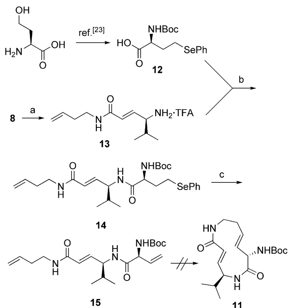
Scheme 5. Attempted synthesis of core macrocycle 11 by using a RCM approach. Reagents and conditions: (a) 1. 1 M aq. LiOH (6 equiv.), MeOH/H 2 O (3:1), 0 °C to room temp. over 30 min; 2. 3-butenylamine hydrochloride (1.1 equiv.), PyBop (1.1 equiv.), DIEA (3 equiv.), DCM, 0 °C to room temp. overnight, 82% (two steps); 3. 20% TFA/DCM, 30 min, >98%; (b) 12 (1 equiv.), 13 (1 equiv.), PyBop (1.01 equiv.), HOAt (1.01 equiv.), DIEA (2.7 equiv.), DCM, from 0 °C to room temp. overnight, 93%; (c) 30% aq. H 2 O 2 /DIEA (1:1), DCM, 50 °C, 3 h, 67%.
