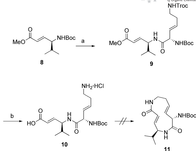
Scheme 3. Attempted synthesis of macrocycle 11 using a macrolactamization approach. Reagents and conditions: (a) 1. 25% TFA/DCM, 30 min; 2. 7 (1 equiv.), PyBop (1.5 equiv.), HOAt (1.5 equiv.), DIEA (2 equiv.), DCM, 0^\circ\text{C} to room temp. overnight, 64% (two steps); (b) 1. Zn (150 equiv.), THF/NH 4 OAc buffer solution 1 M pH 5.0 (5:1), 3 h; 2. 1 M aq. LiOH (2 equiv.), MeOH/H 2 O (3:1), 0^\circ\text{C} to room temp. over 30 min; 3. aq. HCl, 82% (three steps).
