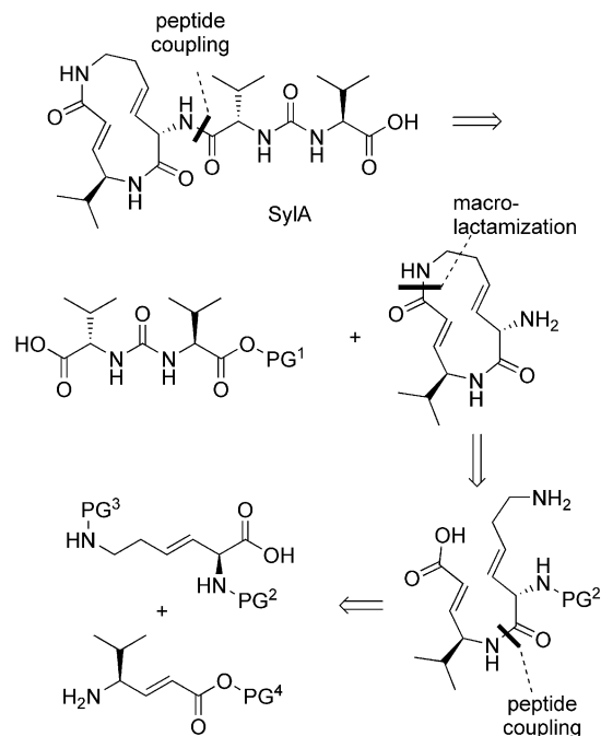
Scheme 1. First retrosynthetic pathway to SylA by using macrolactamization as a key step for ring closure.
