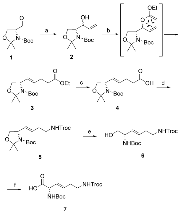
Scheme 2. Synthesis of protected \beta,\gamma -dehydrolysine building block 7 . Reagents and conditions: (a) vinylmagnesium bromide (3 equiv.), THF, 30 min at -78^\circ\text{C} and then 2 h at room temp., 75%, syn/anti , 1:3; (b) triethyl orthoacetate (9 equiv.), propionic acid (0.2 equiv.), xylenes, reflux, 24 h, 90%; (c) 1 M aq. LiOH (3 equiv.), MeOH/H 2 O (3:1), 0^\circ\text{C} to room temp. over 30 min, >98%; (d) 1. diphenyl phosphoryl azide (1 equiv.), Et 3 N (1.2 equiv.), toluene, 30 min at room temp. and then 4 h at reflux; 2. trichloroethanol (3 equiv.) at 50^\circ\text{C} and then 20 h at reflux, 93% (two steps); (e) pyridinium p -toluenesulfonate (PPTS, 0.2 equiv.), MeOH, overnight, reflux, >98%; (f) 1. Dess–Martin periodinane (2 equiv.), DCM, 2 h, 0^\circ\text{C} ; 2. aq. NaClO 2 (7 equiv.), aq. NaH 2 PO 4 (4 equiv.), t BuOH/2-methyl-2-butene (3:1), 0^\circ\text{C} to room temp. over 30 min, 69% (two steps).
